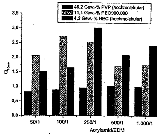
Fig. 6: Swelling experiments of acrylamide/ethylenedimethacrylate hydrogels incorporating different rheological additives
